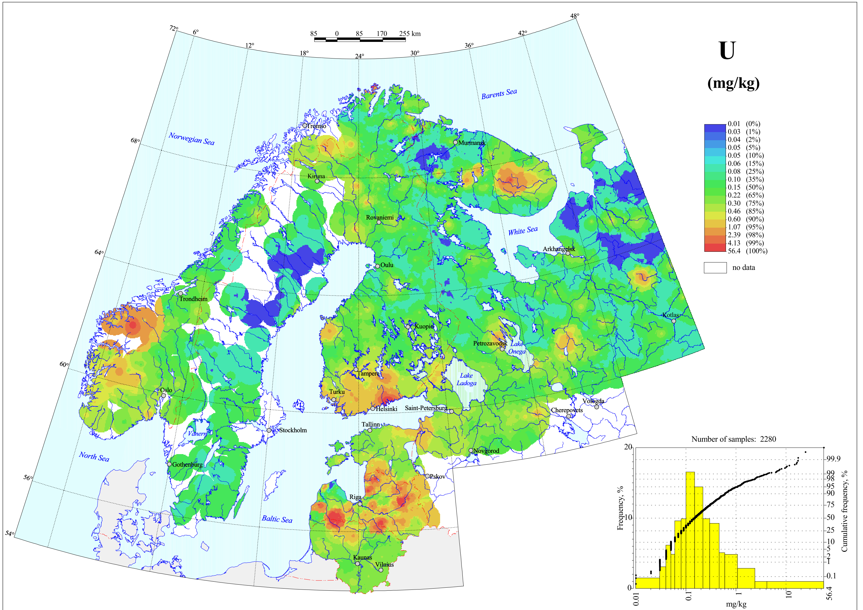
Uranium in Organic Soil Layer, Total Content
